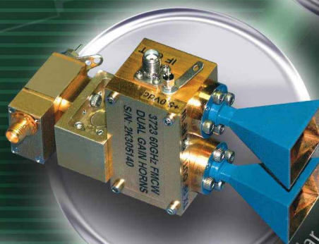
60 GHz FMCW Radar
