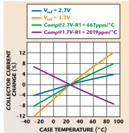
▲ Fig. 3 Current mirror circuit temperature stability.
