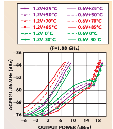
▲ Fig. 17 Low V_{cc} voltage ACPR test results for the proposed circuit.
