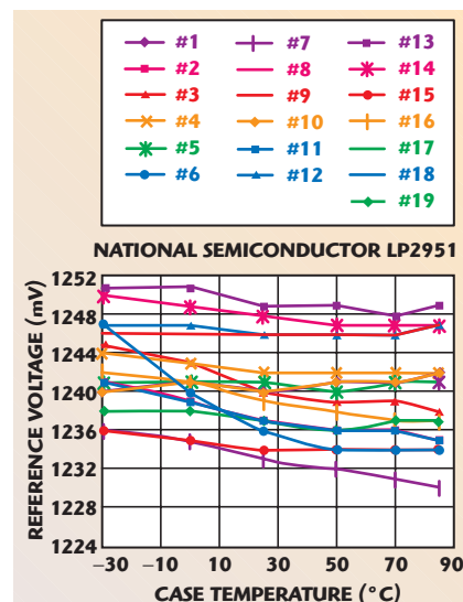
▲ Fig. 19 Several LDO test results over temperature.
