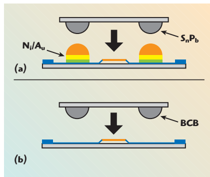
▲ Fig. 2 Schematic picture of (a) metal/solder sealing and (b) polymer (BCB) sealing of MEMS switches.
