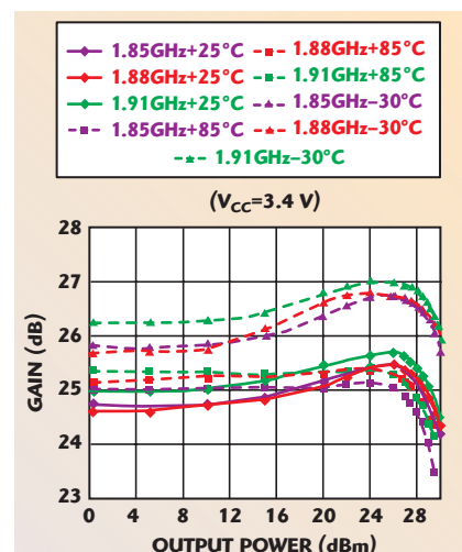
▲ Fig. 12 Gain test results for the proposed circuit at room and extreme temperatures.
