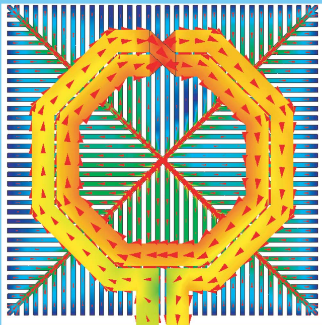
Current Distribution Visualization on a RFIC Cell
