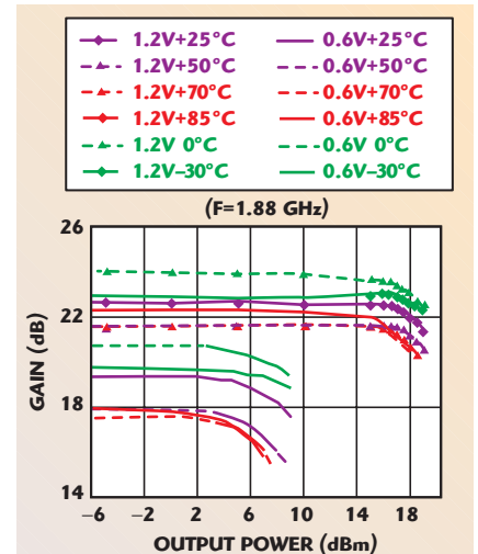
▲ Fig. 16 Low V_{cc} voltage gain test results for the proposed circuit.
