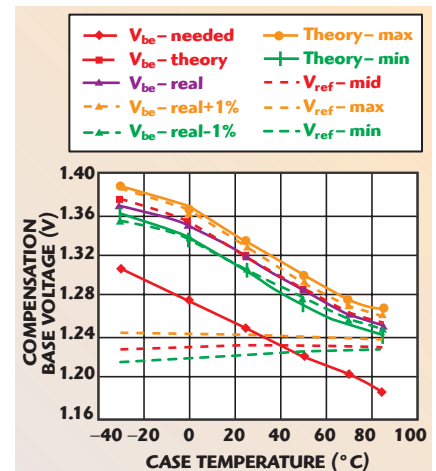
▲ Fig. 8 Base control voltage test and simulation results.
